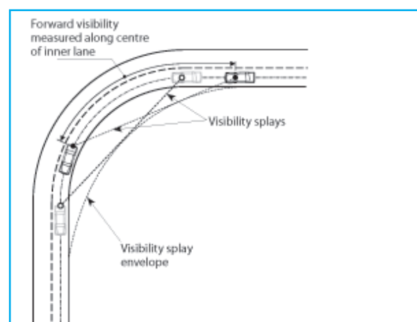
Figure 10.1 - Measurement of forward visibility
